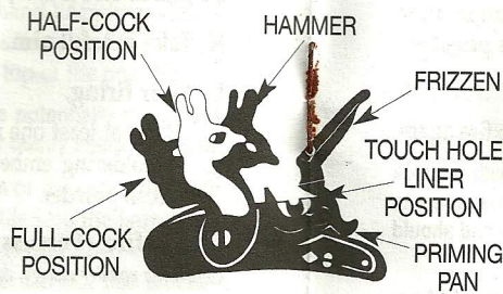
Flintlock: External Lock Parts
