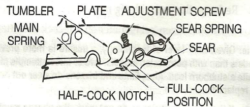
Internal Lock Parts
