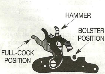
Percussion: External Lock Parts
